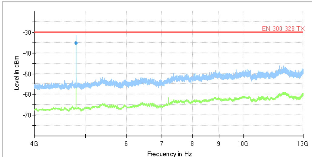
Diagram, Peak overview sweep, 4 GHz – 13 GHz, TX low channel. Emissions below 4000 MHz are attenuated by a high-pass filter.
