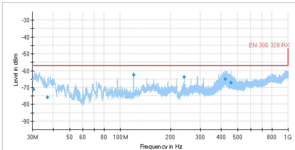
Diagram, Peak overview sweep, 30 MHz – 1000 MHz, RX low channel
