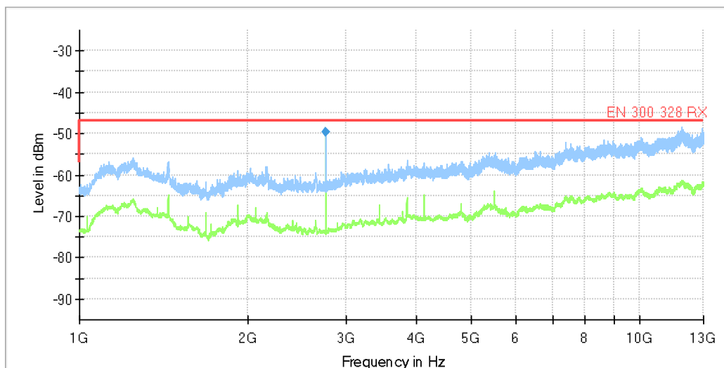
Diagram, Peak overview sweep, 1 GHz – 13 GHz, RX high channel
