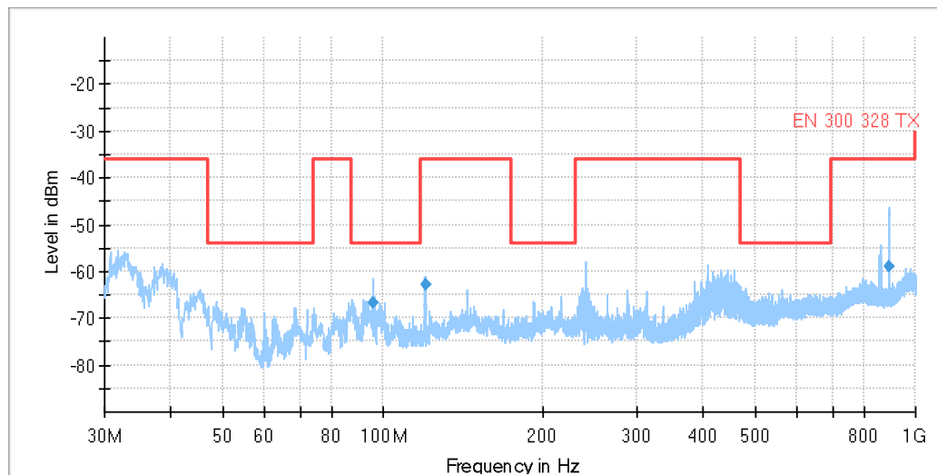
Diagram, Peak overview sweep, 30 MHz – 1000 MHz, TX low channel
