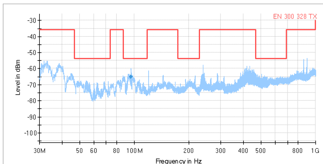
Diagram, Peak overview sweep, 30 MHz – 1000 MHz, TX high channel
