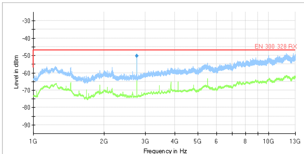
Diagram, Peak overview sweep, 1 GHz – 13 GHz, RX low channel
