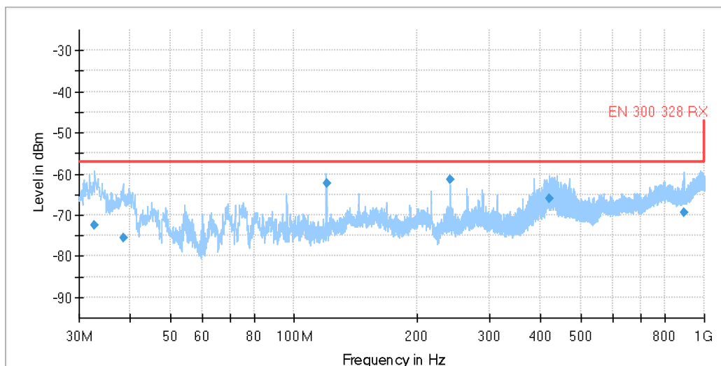
Diagram, Peak overview sweep, 30 MHz – 1000 MHz, RX high channel
