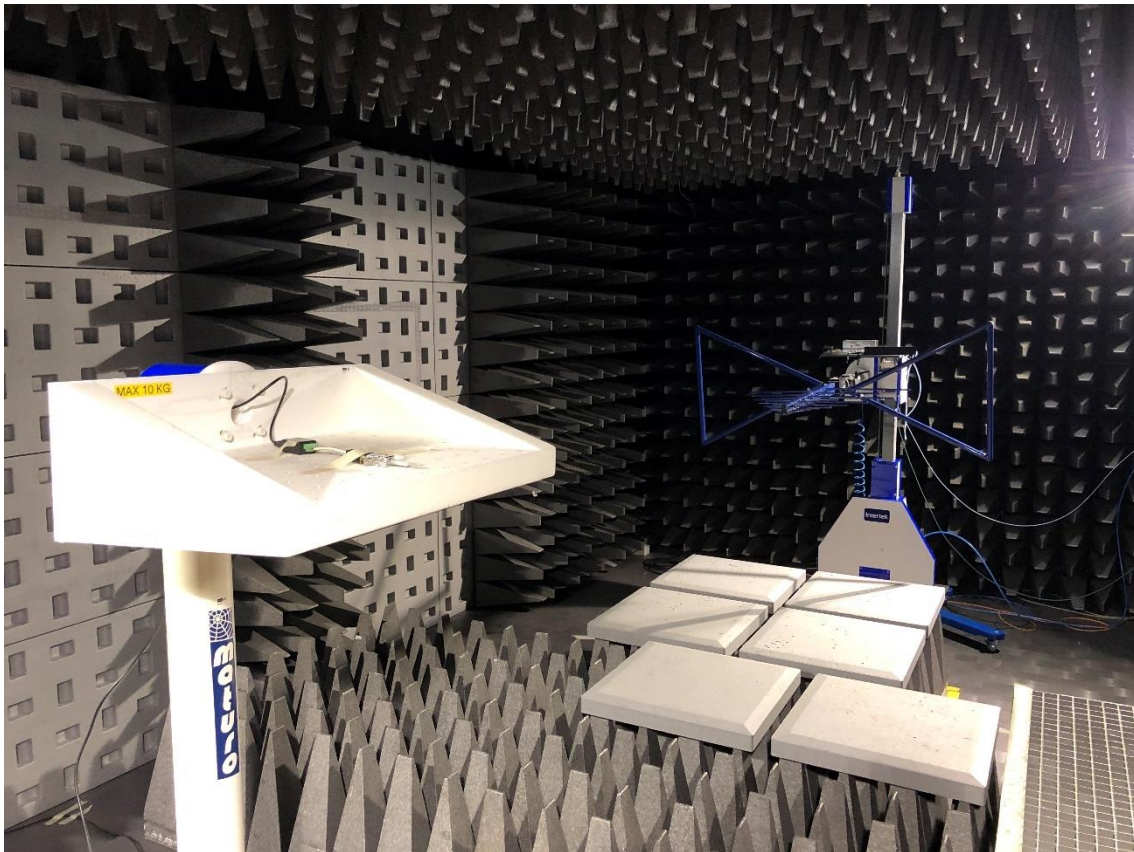
Photo of the test set-up for radiated emission 30 – 1000 MHz
