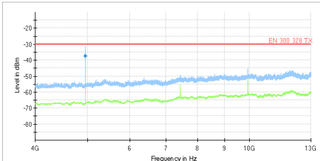
Diagram, Peak overview sweep, 4 GHz – 13 GHz, TX high channel. Emissions below 4000 MHz are attenuated by a high-pass filter.
